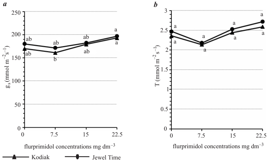
Fig. 5. Effect of flurprimidol applied as single, foliar spray on stomatal conductance to water vapor ( g_s ) (a) and transpiration rate (T) per unit leaf area (b) of “Kodiak” and “Jewel Time” chrysanthemums. Data averaged over two growing seasons. The means indicated by the same letter do not differ significantly at p = 0.05 , according to Duncan’s multiple range test
